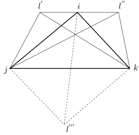
Fig. 4. An example of \Delta ijk and node l .
