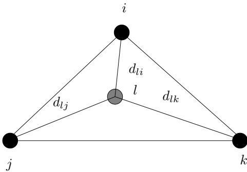
Fig. 1. An illustrative example for the barycentric coordinate.
