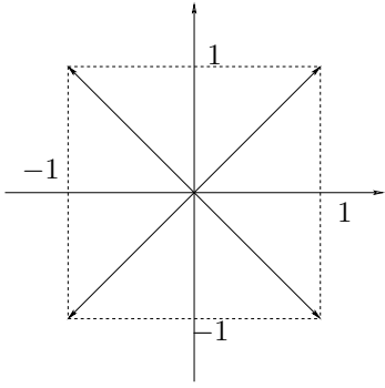
Fig. 3. An illustration for the necessity proof.
