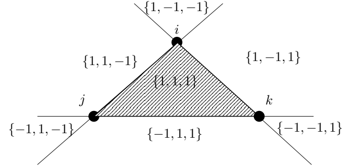
Fig. 2. Seven possible sign patterns for \{\sigma_{li}, \sigma_{lj}, \sigma_{lk}\} .
