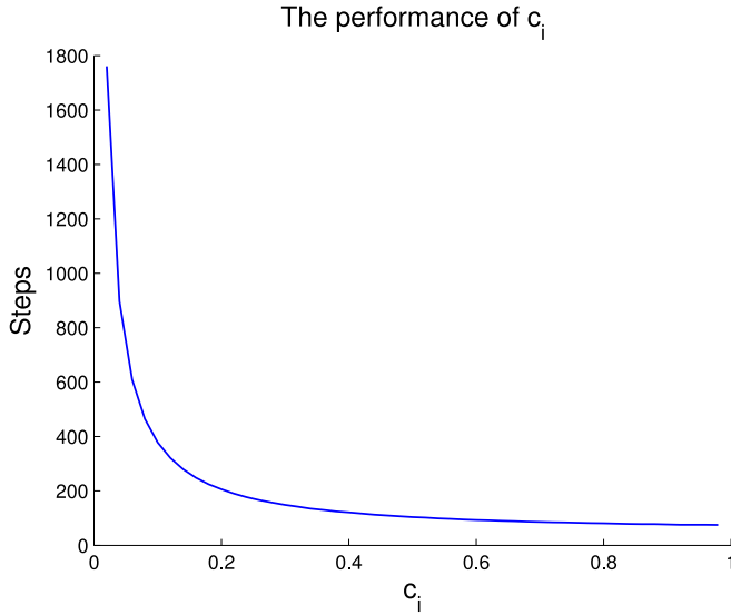
Fig. 5. The number of iterations ( y -axis) for different c_i until \|x(k) - x^*\| < 0.05 .
