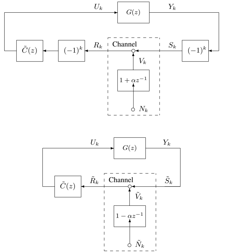
Fig. 3. Original LTV scheme (top) and equivalent interpretation (bottom)
