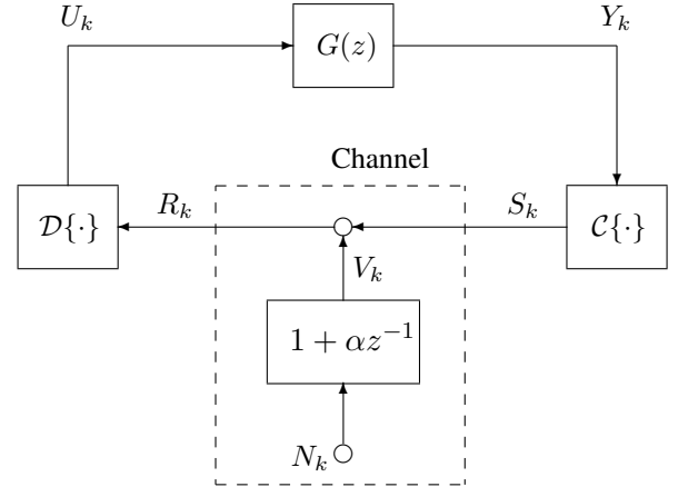
Fig. 2. Feedback stabilization over a communication channel
