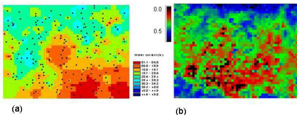
Figure 2.3: (a) Top 6 cm volumetric soil water content ( \text{cm}^3 \text{cm}^{-3} ) distribution within the validation area for Campaign-2 (b) Disaggregated near surface water content ( \text{cm}^{-3} \text{cm}^{-3} ) for the validation area on 2 May 2004.
