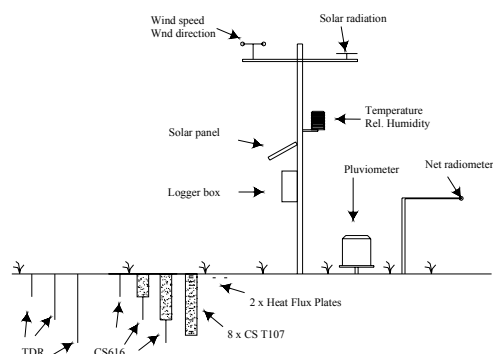
Figure 6. Typical setup for the climate stations.
