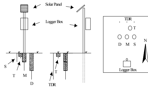
Figure 5. Typical setup of a soil moisture monitoring site (front view, side view and top view); showing shallow (S), medium (M), and deep (D) CS616 and the CS T107 (T) sensors.
