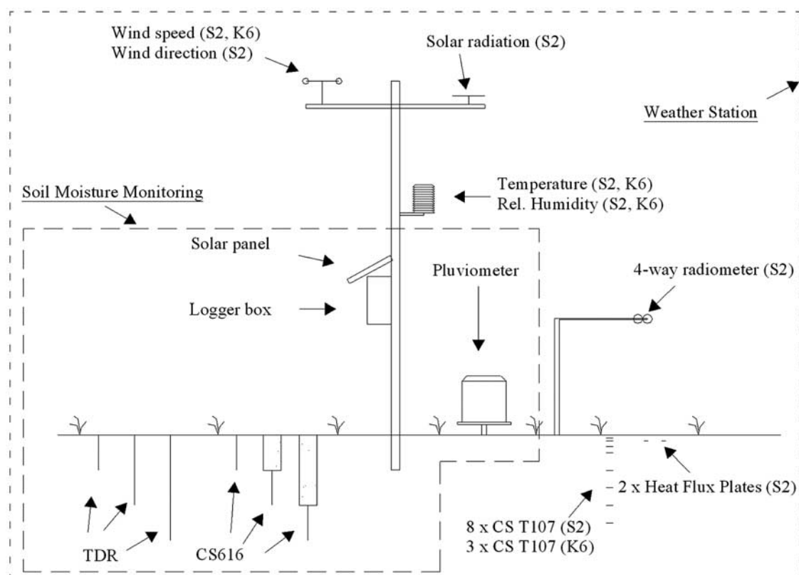
Figure 7. Schematic of the weather and soil moisture stations. The larger box includes the instrumentation typically installed at weather stations, while the smaller box includes the instruments typically installed at soil moisture monitoring sites. Instruments annotated with S2 are located at the AWS at Stanley, and those with K6 are located at the AWS at Spring Hill.
